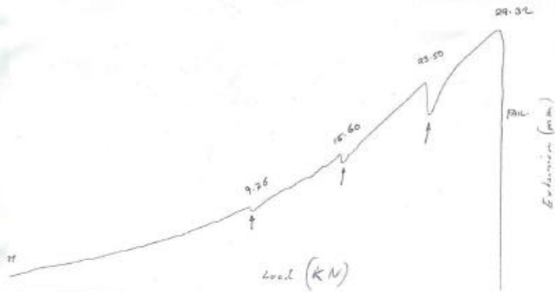
Tape Knot in 25mm Tube Tape Load extension Curve CIT machine
