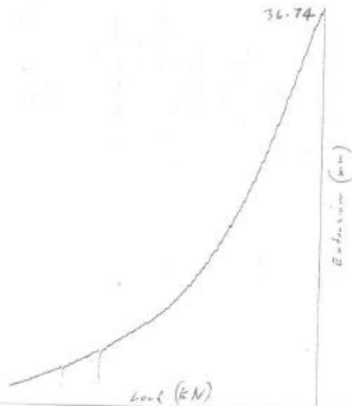
Double Fisherman's Knot in 9mm static rope Load extension Curve ADFA machine
