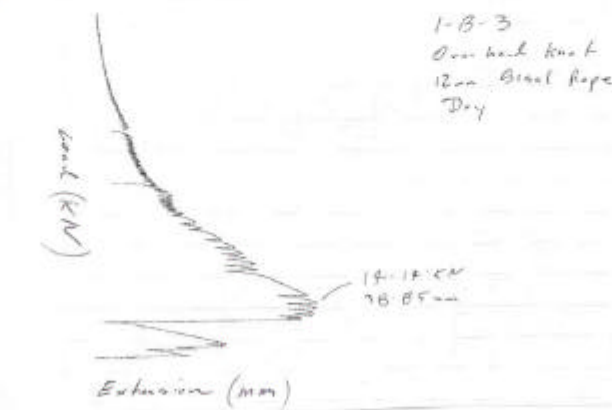
Overhand Knot in 12mm Sisal rope Load extension curve ADFA machine
