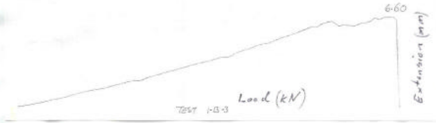
Overhand Knot in 25mm tube tape Load extension curve CIT machine
