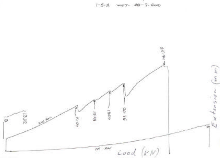
Alpine Butterfly Knot in 11mm static rope Load extension curve CIT machine
