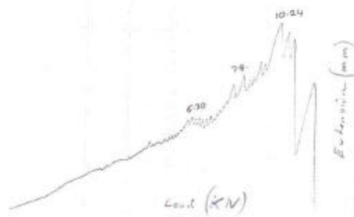
Double Fisherman's Knot in 10mm Sisal rope Load extension Curve ADFA machine
