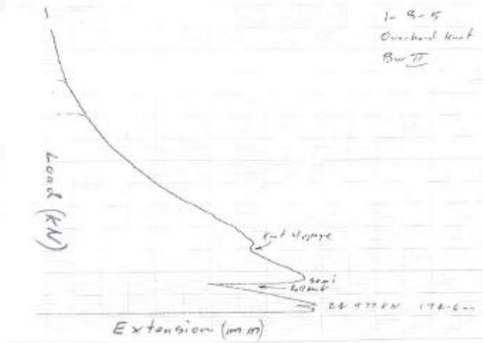
Overhand Knot in 11mm static rope Load extension curve ADFA machine
